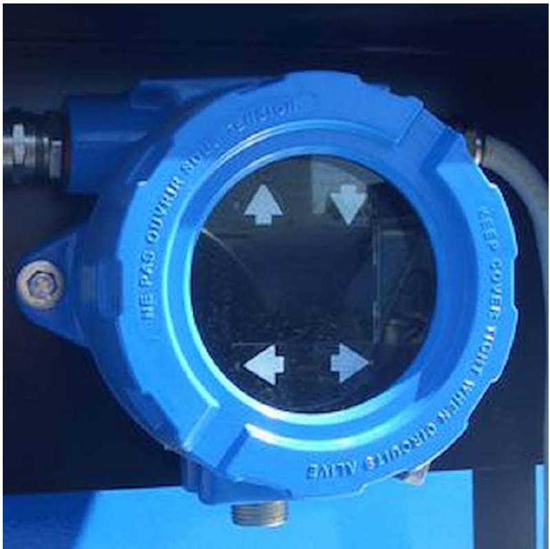
DIGIMAG level gauge (inox float).
